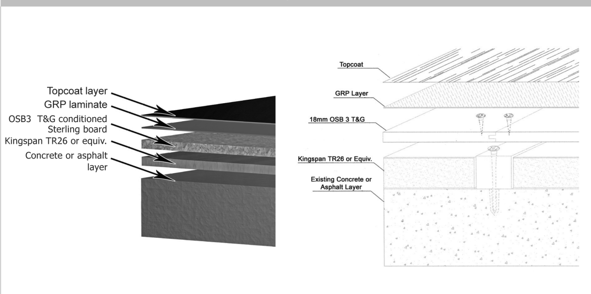
Cross-section of Warm Roof onto Concrete or Asphalt
